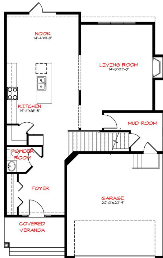
MAIN FLOOR 989 Sqft
