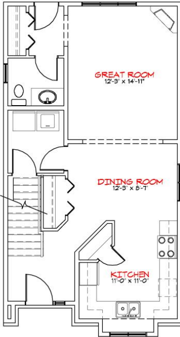
MAIN FLOOR 704 SQ FT
