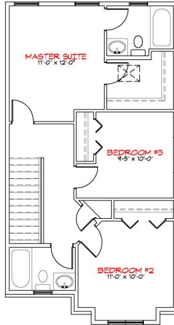
SECOND FLOOR 682 SQ FT
