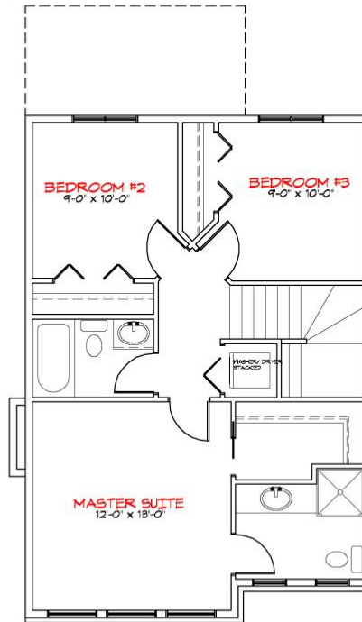
SECOND FLOOR 640 SQ FT
